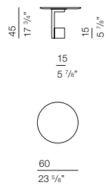
CUB001 coffee table ø60 H45
