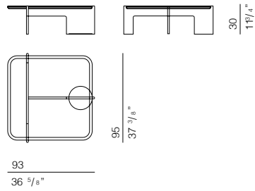
PREST7 squared low table with top 90x90 H30
