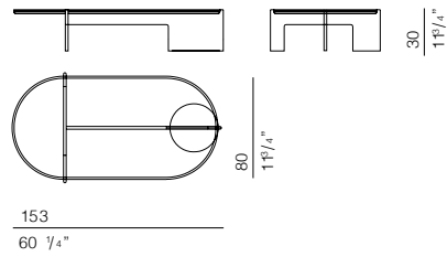
PREST6 oval low table with top 75x150 H30
