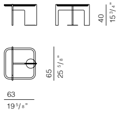
PREST2 low table with top 60x60 H40
